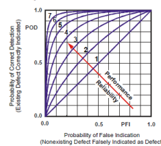
Comparison of Different NDT-Systems
